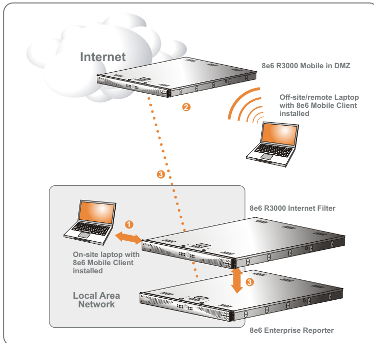
Diagram illustrates how a mobile laptop is 1 filtered by the on-site/local R3000 Internet filter, and by the 2 remote R3000 Mobile in the DMZ when off-site. In addition, the laptop's internal and remote Web activity logs are 3 sent to the on-site Enterprise Reporter for reporting and archiving.
